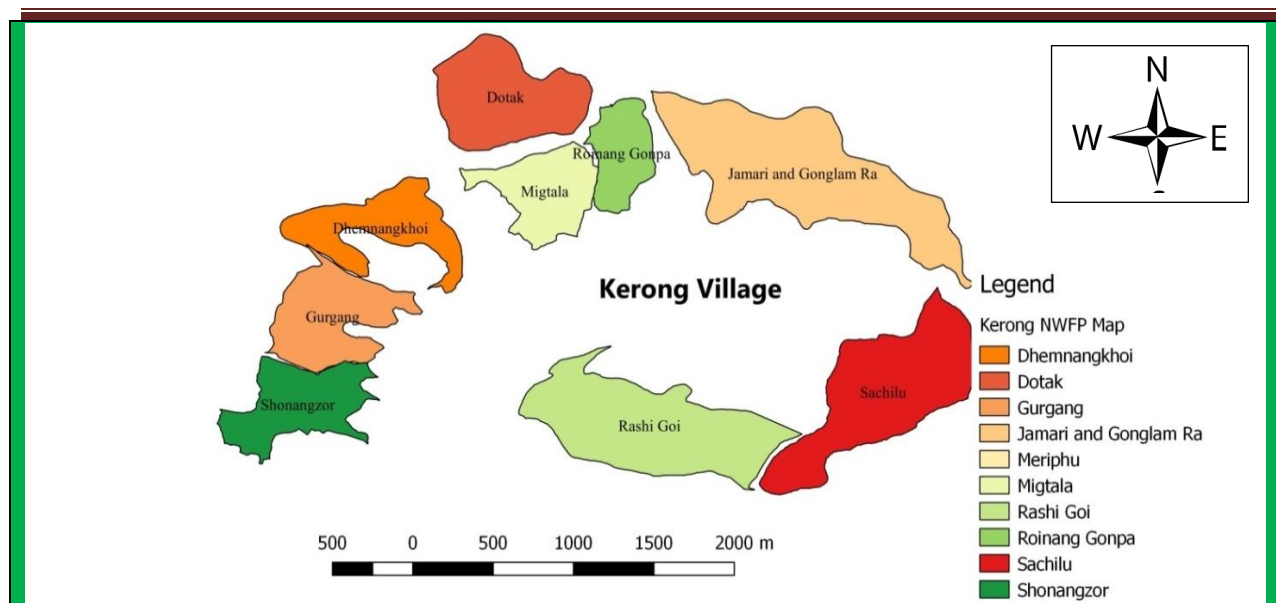
Figure 2. Sketch map of NWFP collection area
